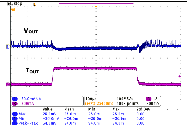
FIG.8 TRANSIENT RESPONSE (3.8VIN, 0% to 100% LOAD STEP, MODE=GND)
