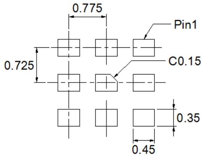
RECOMMENDED STENCIL PATTERN BASED ON 130µm THICKNESS STENCIL
