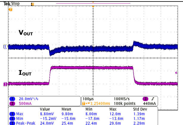
FIG.7 TRANSIENT RESPONSE (3.8VIN, 0% to 100% LOAD STEP, MODE=VIN)
